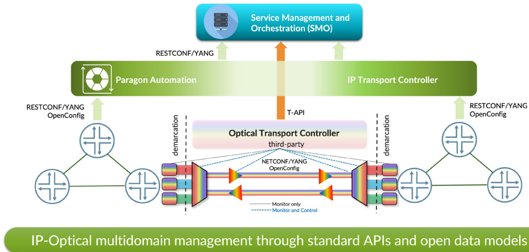
Figure 6. Paragon Automation enables multilayer visibility and support
