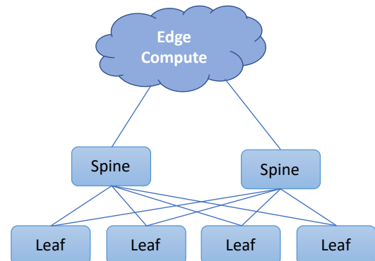
Spine-Leaf Network
