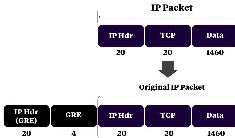
Figure 3. GRE Encapsulation
