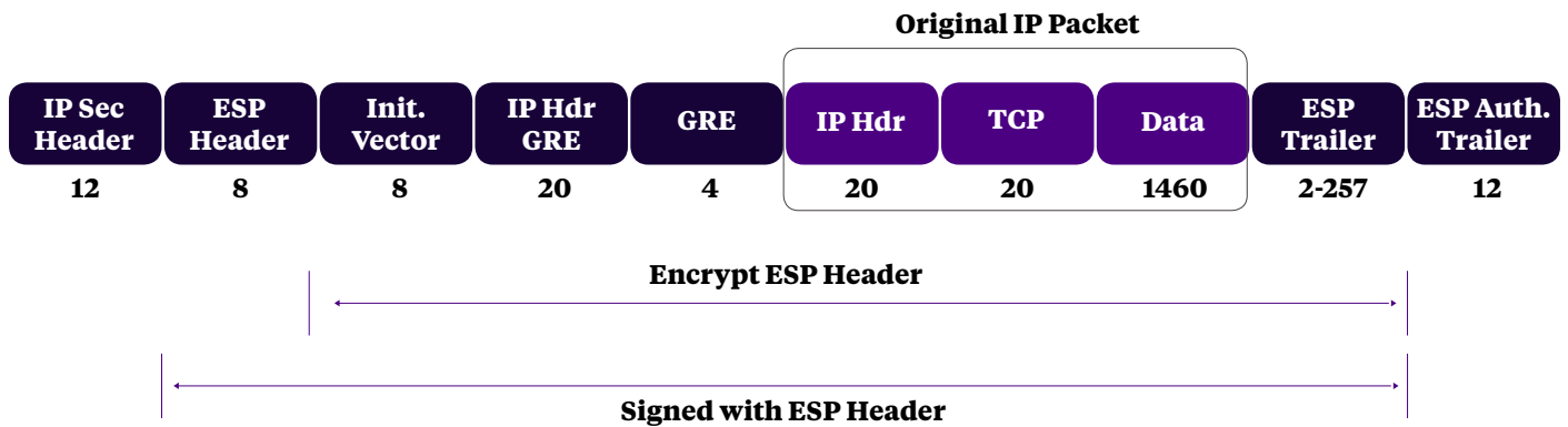
Figure 4. IPsec Encapsulation
